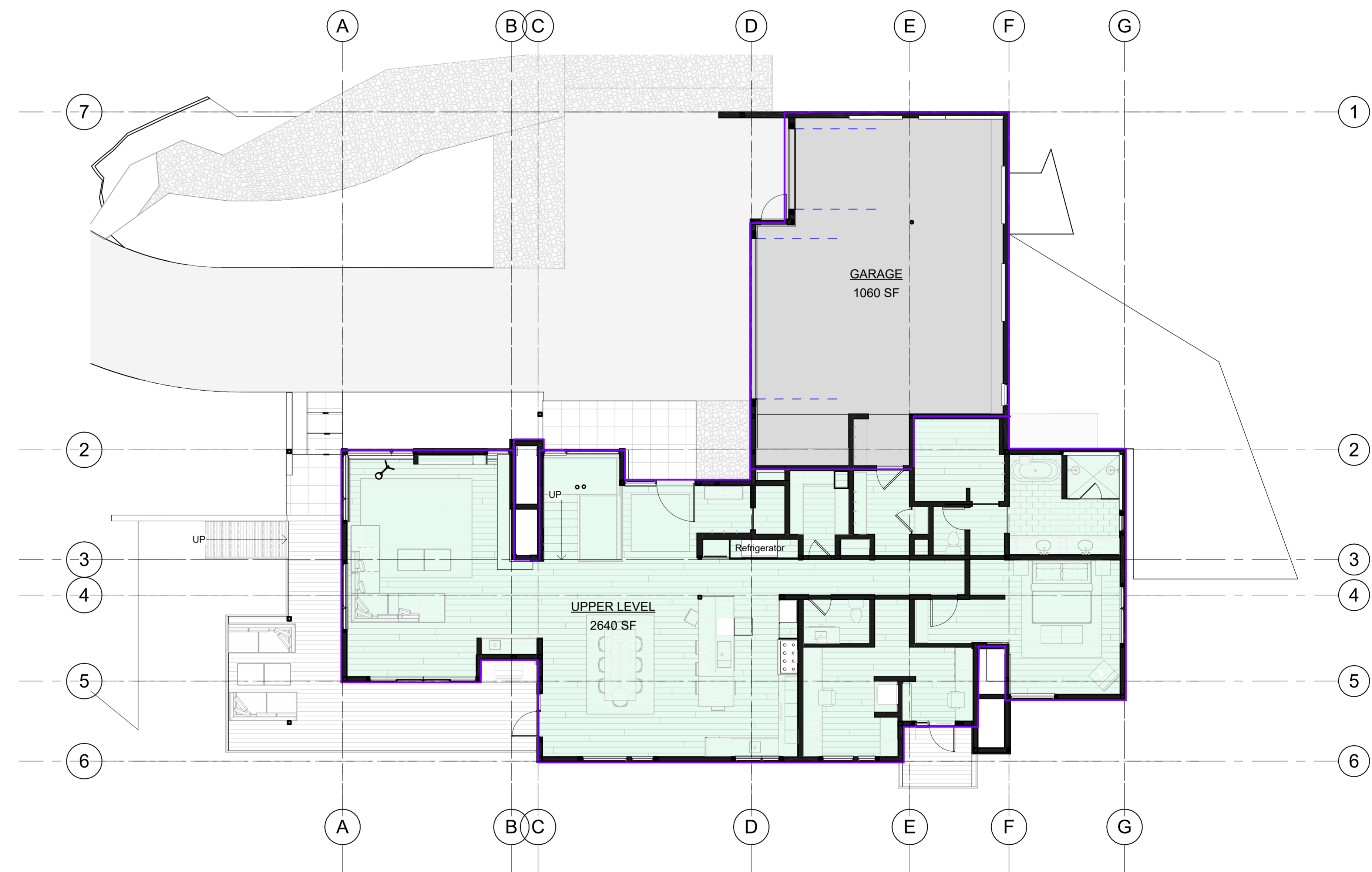
2 MAIN LEVEL - AREA PLAN A070 1/8" = 1'-0"
